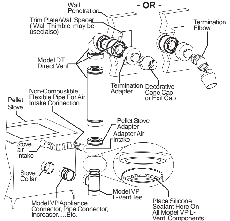
Through the Wall Installation
