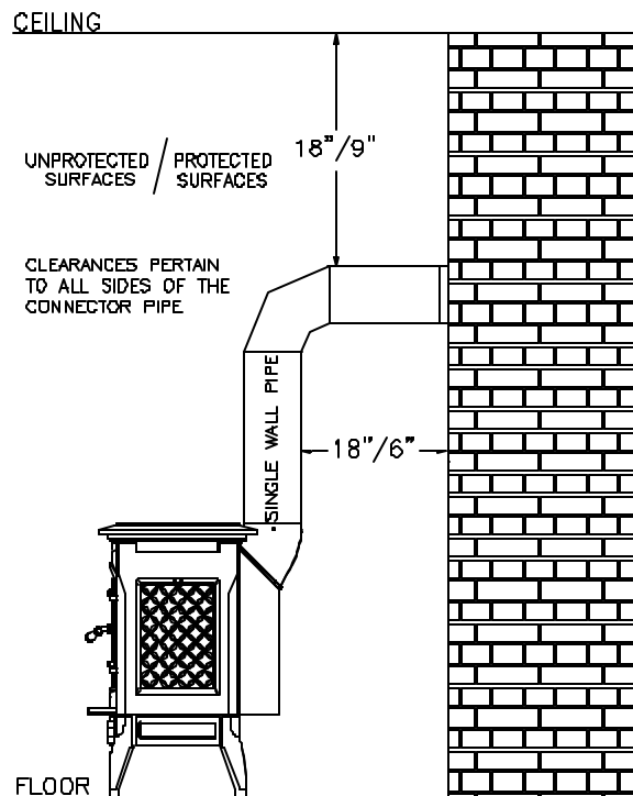
SINGLE WALL CONNECTOR
