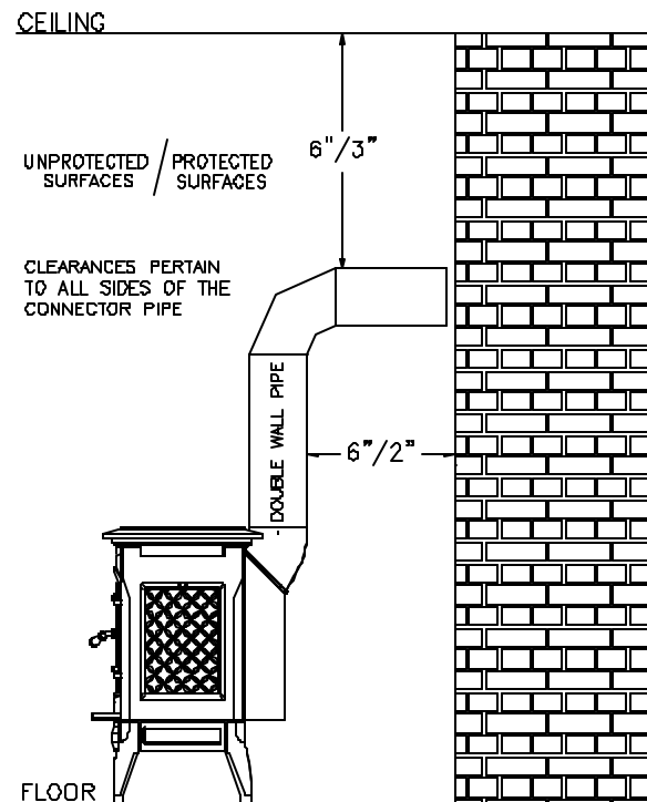
DOUBLE WALL CONNECTOR
