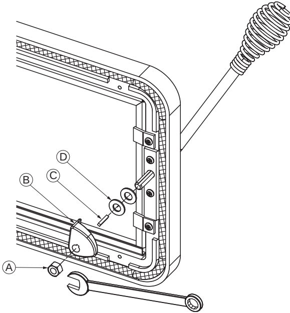
Figure 20: Removing the door latch
