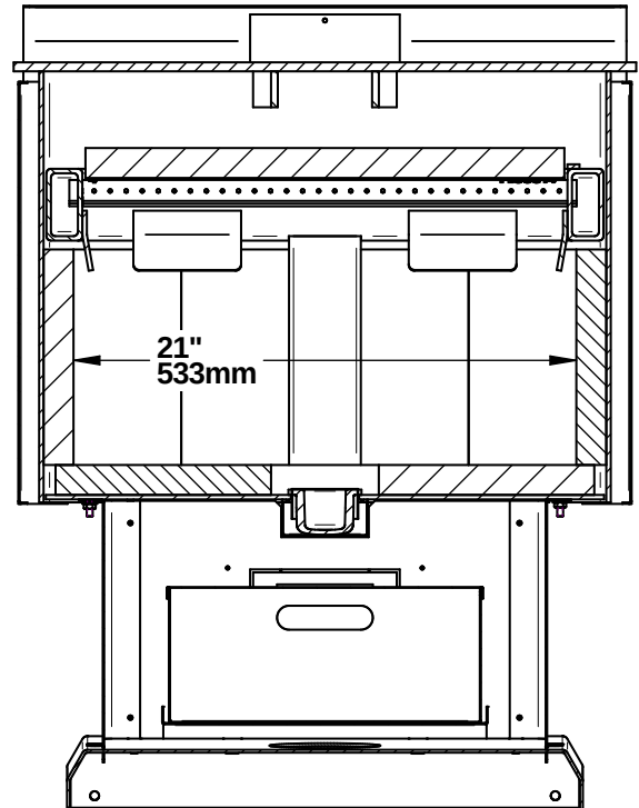
Figure 14: Front view - Combustion chamber
