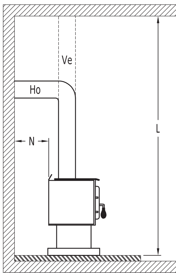
Figure 24: Clearances - Top
