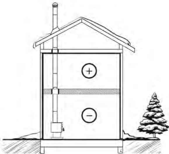
Figure 32: Good System Design
