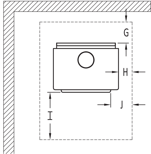
Figure 26: Floor Protection
