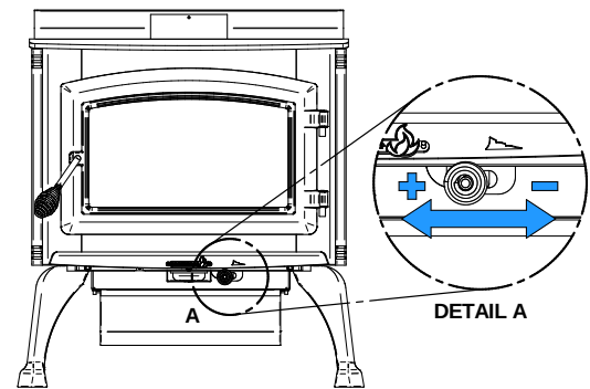
Figure 19: Air Intake Control
