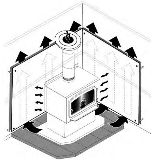
Figure 28: Heat shield
