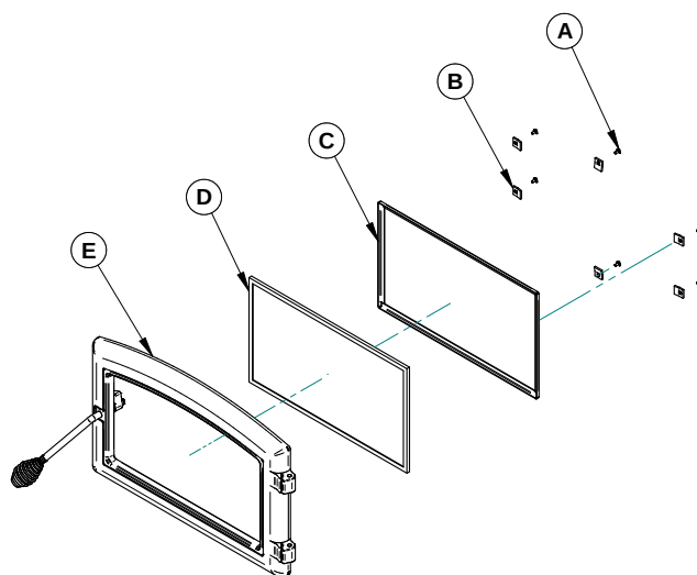
Figure 22: Replacing the glass
