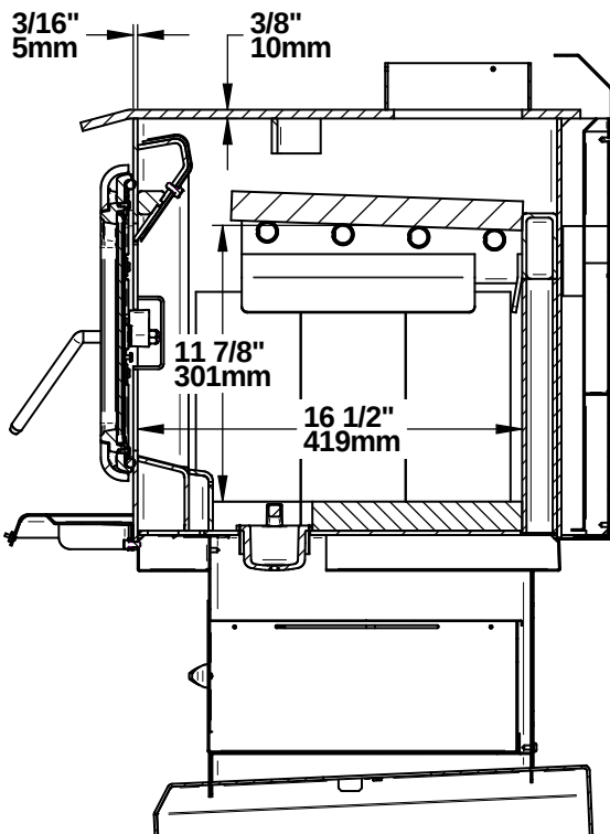
Figure 15: Side view - Combustion chamber
