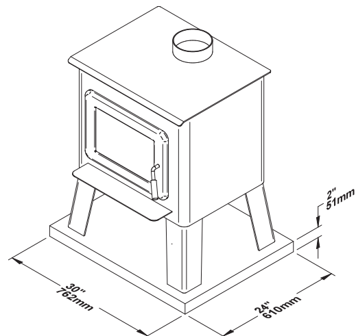
Figure 27: Floor protection in a mobile home
