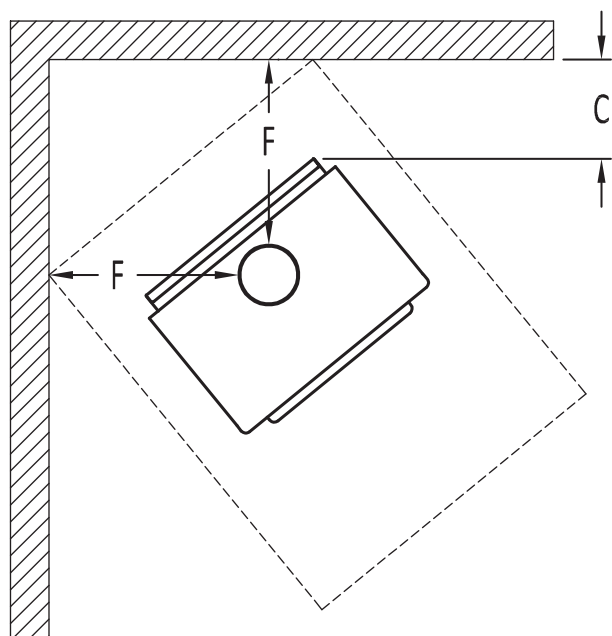
Figure 25: Clearances - Corner
