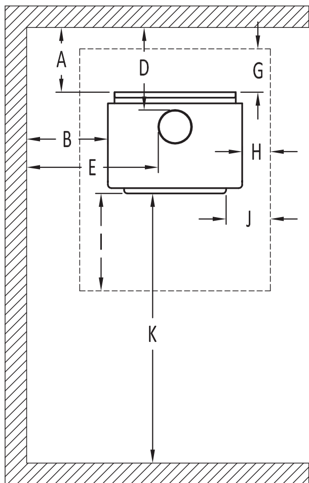
Figure 23: Clearances -Side
